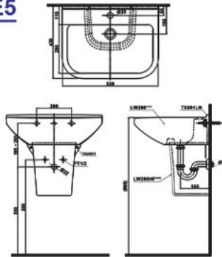
Wall Hung Lavatory 500W X 350D X 820H mm
