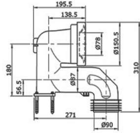
Slip-In Connector for S-Trap Toilet
